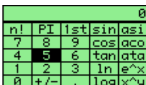
Figure 11.46.: Calculator
